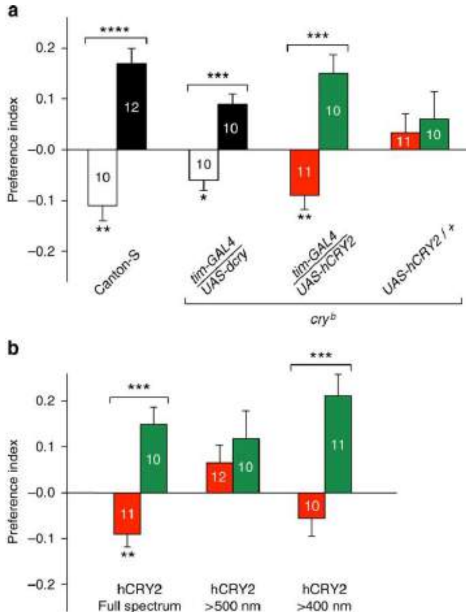
(a) A tim-GAL4 -driven human CRY2 transgene ( tim-GAL4/UAS-hCRY2 ) rescues magnetic responses in the CRY loss-of-function cry b mutant background. For comparison, naive and trained responses to the
