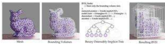
Figure 1: We present a fast encoding of bounding volume hierarchies (BVH) for broad-phase collision detection with low-memory usage. Our method can generate trees supporting canonical indexing of implicit trees without the need for padding memory. We achieve this by observing that for a given number of objects, an almost-perfect binary tree can be completely determined, and the nodes missing for it to be "perfect" can be characterized through simple bit-manipulations. The figure shows a sequence where a BVH is constructed over a mesh using our novel representation. A minimal number of nodes are stored which can be indexed like the heap data structure.
