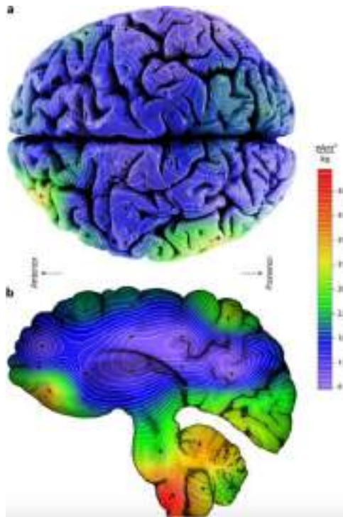
A map of magnetite concentrations in the brain.
